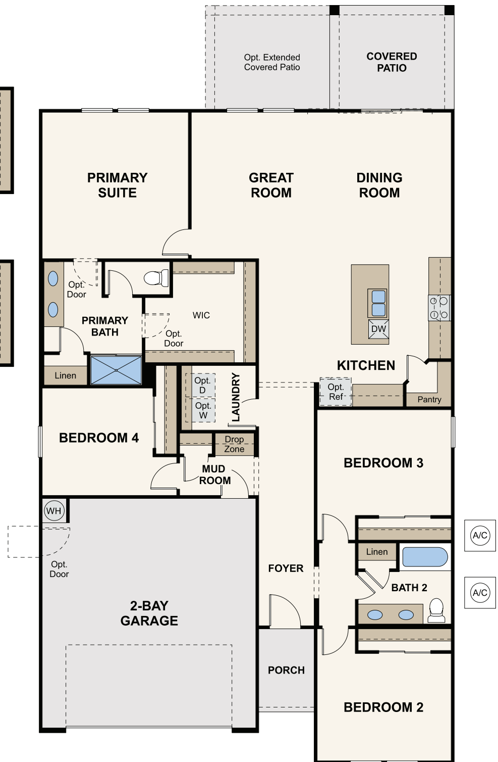
FLOOR PLAN
